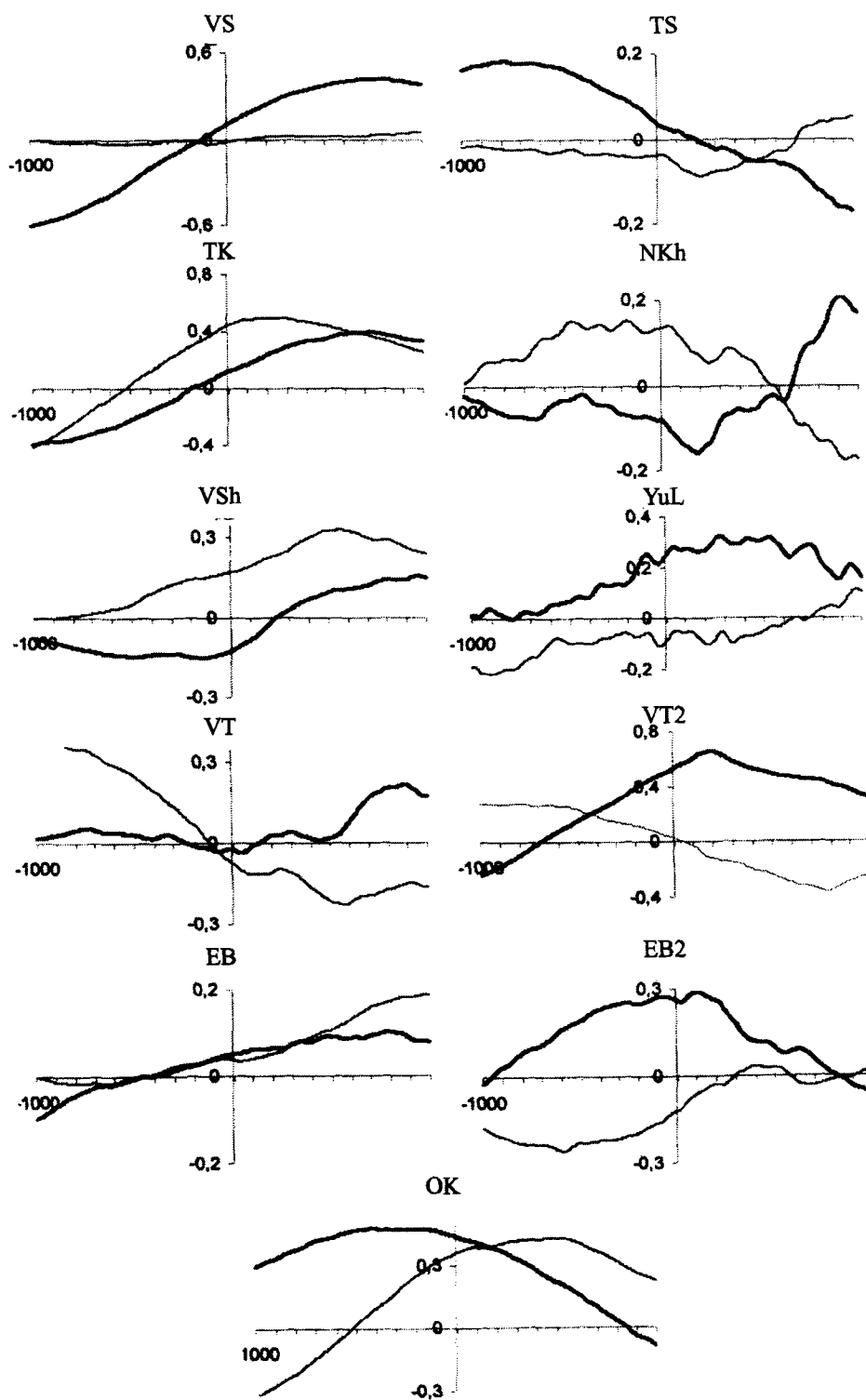
Fig. 2. Cross-correlation functions between fluctuations of the pressure center in the frontal (bold lines) and sagittal (thin lines) planes and eye movements during slow tracing for different volunteers.
